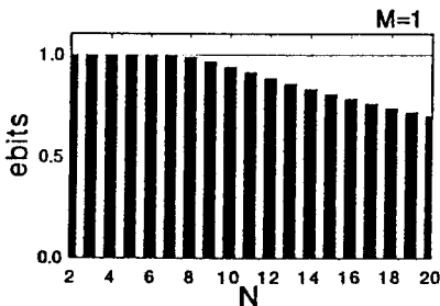
FIG. 3. The maximum values of the entanglement E^{N,1} as a function of the total number N of quantum dots in systems with single excitation. On the scale of the figure, \max_t E^{7,1}(t) = 0.9997 does not differ from unity. However, for higher values of N , a monotonous decrease of the maximum entanglement is clearly visible.
