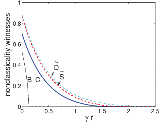
FIG. 2. (Color online) An example of the environment-induced sudden vanishing of the nonclassicality witnesses for two noninteracting modes. The damping model is described in Sec. IV for the initial Werner-like state \rho_1 with p = 0.8 . Key: the concurrence C (solid curve), nonlocality B (dotted curve), and two witnesses describing the photon-number-difference correlations: \tilde{S} (dashed curve) for S_0 = 0.03 and \tilde{D} (dot-dashed curve) for D_0 = 0.1 .
