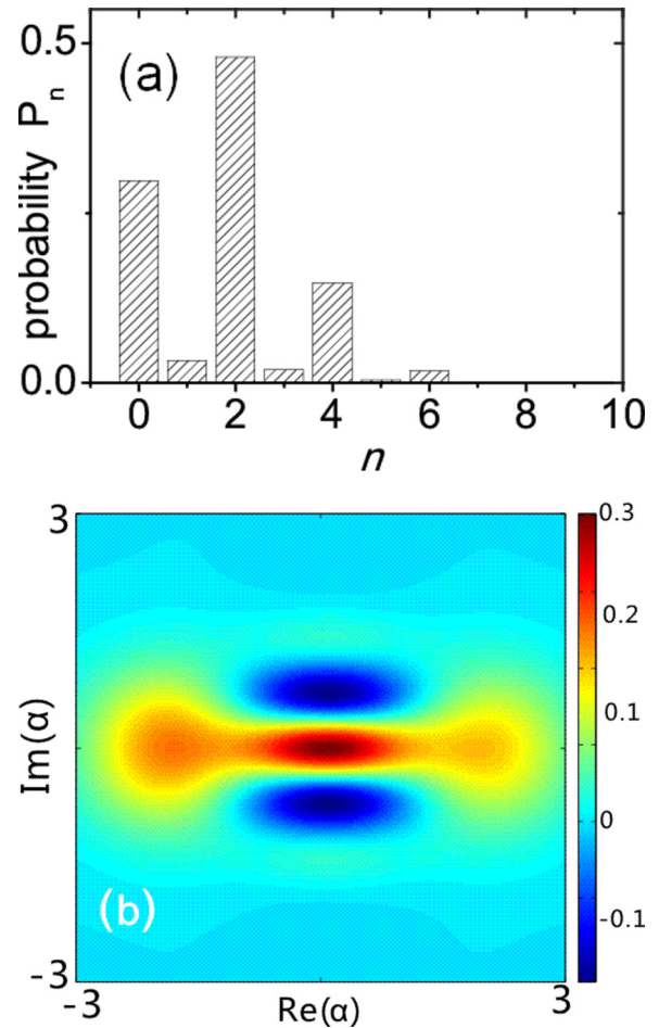
FIG. 4. (a) The phonon-number (Fock-state) distribution and (b) the Wigner function W(\alpha) for the Schrödinger-cat-like state generated at the evolution time t_{\max} = 27.5 \mu\text{s} [indicated by the vertical dashed line in Fig. 3(a)] corresponding to the maximum of the fidelity F . Other parameters are the same as in Fig. 3(a).
