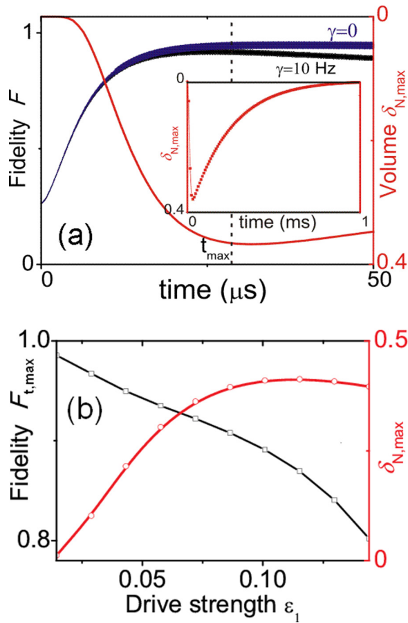
FIG. 3. (a) Time evolutions of the target-state fidelity F for the mechanical decaying and nondecaying cases, and the nonclassical volume \delta_N . The inset shows the evolution of \delta_N in a much longer time scale. (b) The maximum fidelity F_{t,\max} and the nonclassicality volume \delta_{N,\max} vs the resonant driving strength \epsilon_1 . The vertical dashed line in (a) indicates t_{\max} = 27.5 \mu\text{s} corresponding to the maximum of F . In panel (a) we assume \epsilon_1/(2\pi) = 5 MHz and \lambda = 0.06 , corresponding to the quadratic coupling strength \Theta_c/(2\pi) = 2\lambda^2\epsilon_1 = 36 KHz. The other parameters are \Gamma/(2\pi) = 0.4 MHz, n_{\text{th}} = 5 , \gamma/(2\pi) = 10 Hz, and \epsilon_2/(2\pi) = -72 KHz.
