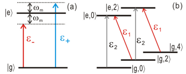
FIG. 2. Schematic diagrams showing how to cool down and engineer the mechanical mode of the CNT into (a) a squeezed state and (b) a macroscopically distinct coherent-state superposition (i.e., a Schrödinger-cat-like state).
