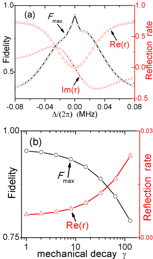
FIG. 5. (a) The highest fidelity F_{\max} , dispersion rate \text{Im}(r) , and reflection rate \text{Re}(r) , vs (a) the detuning \Delta_d and (b) the mechanical decay rate \gamma . In (b), since \text{Im}(r) \ll \text{Re}(r) , \text{Im}(r) is not shown. Other parameters are the same as those in Fig. 3.
